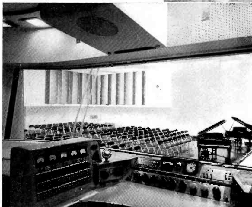
CBS, New York. Here is a specially designed auditorium-type studio control console complete with monitoring and program amplifier equipment. It represents one of several such consoles used in CBS's expansive installation, custom-built by RCA. Control of 8 input circuits (6 microphone circuits and two remote lines) is provided. Mechanical design affords unobstructed studio view.
