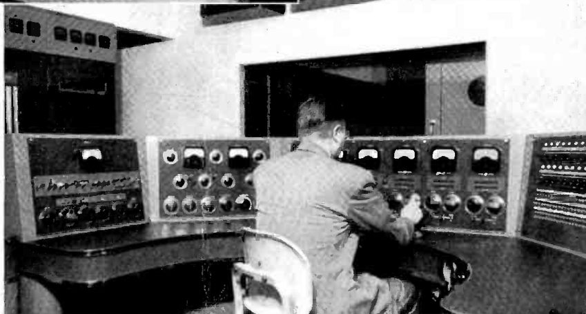
CBS, New York. Here is a specially designed auditorium-type studio control console complete with monitoring and program amplifier equipment. It represents one of several such consoles used in CBS's expansive installation, custom-built by RCA. Control of 8 input circuits (6 microphone circuits and two remote lines) is provided. Mechanical design affords unobstructed studio view.
